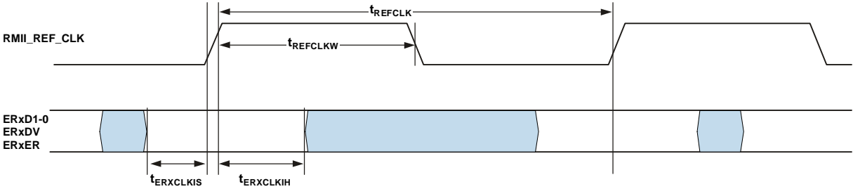
Figure 30. 10/100 Ethernet MAC Controller Timing: RMI Receive Signal
